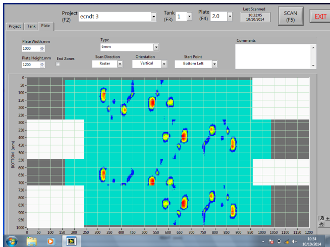
Figure 1: TruFlux Raster Scan
